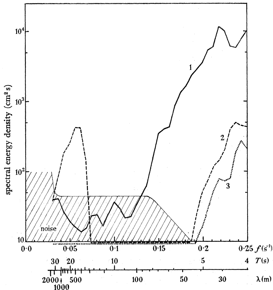
FIGURE 9. Wave spectra in shore lead. 1, 75.5^\circ \text{S} , 20 knot wind; 2, 71.1^\circ \text{S} , calm; 3, 75.5^\circ \text{S} , calm.
