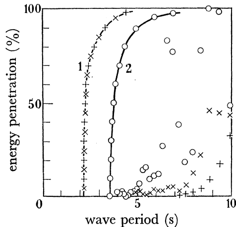
FIGURE 11. Energy penetration into a broken ice field. Some theoretical estimates and observed values with smaller floes. Theoretical curves (Shapiro & Simpson): 1, ice 1.2 m thick; 2, ice 3 m thick. Observations: \circ , 3 m thick, 10 m diam. ( 57.5^\circ S); \times , 1 m thick, 20 m diam. ( 65.0^\circ S); + , 1 m thick, 20 m diam ( 67.4^\circ S).
