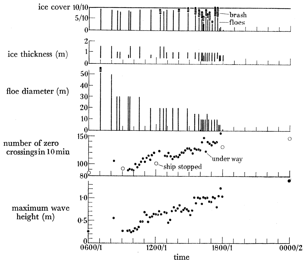
FIGURE 10. Wave and ice data from continuous record made with ship under way, lat. 67.7^{\circ} S to lat. 66.1^{\circ} S, return voyage.
