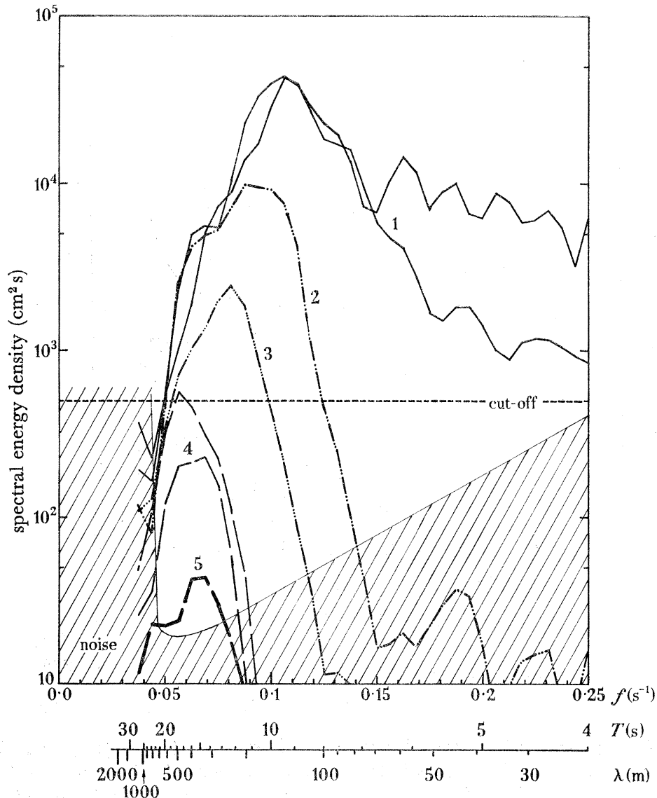
FIGURE 8. Wave spectra during return voyage. 1, Open ocean ( 66.1 and 66.9^\circ S); 2, floes 20 m diam. ( 67.4^\circ S); 3, floes 30 m diam. ( 67.6^\circ S); 4, floes 1 to 5 km diam., \frac{1}{4} to 1 m thick ( 67.9 and 68.2^\circ S); 5, floes 1 km diam., \frac{1}{2} to 1\frac{1}{2} m thick ( 67.8^\circ S).
