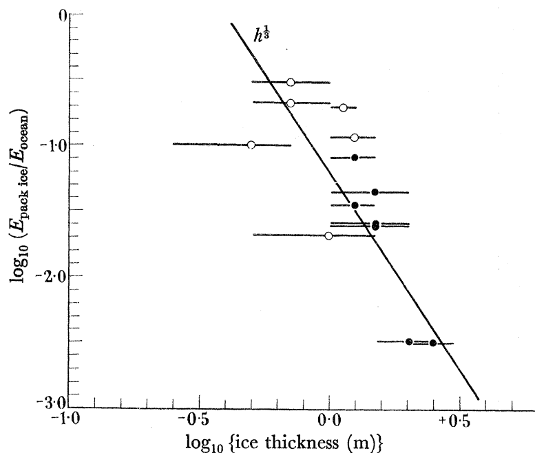
FIGURE 15. Energy penetration into fields of large ice floes as a function of ice thickness. ●, Outward journey; ○, return journey.
