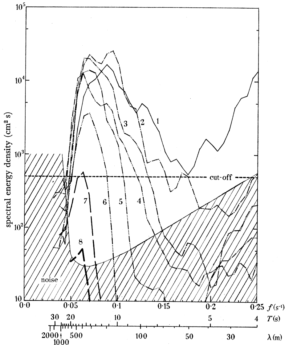
FIGURE 7. Wave spectra during outward voyage. 1, Open ocean ( 64.2^{\circ} S); 2, floes 10 m diam. ( 61.9^{\circ} S); 3, floes 20 m diam. ( 66.5^{\circ} S); 4, floes 30 m diam. ( 65.8^{\circ} S); 5, floes 40 m diam. ( 67.1^{\circ} S); 6, floes 50 m diam. ( 67.7^{\circ} S); 7, floes 3 km diam., 1 to 1\frac{1}{2} m thick ( 68.8^{\circ} S); 8, floes 5 km diam., 2 to 3 m thick ( 70.3^{\circ} S).
