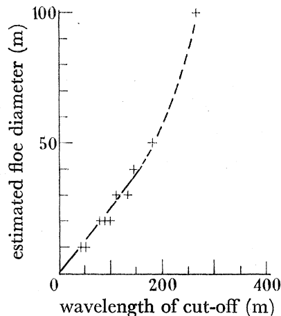
FIGURE 12. Floe diameters and wavelength of cut-off with smaller floes.
