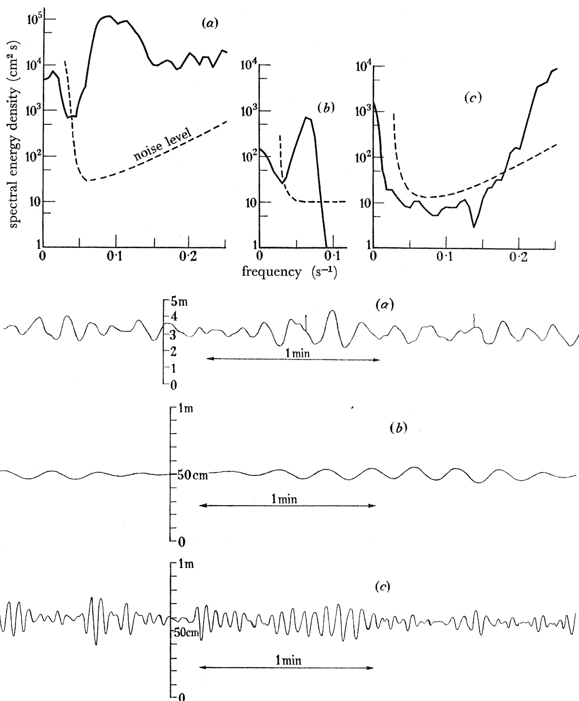
FIGURE 1. Wave records and wave spectra. (a) Open ocean, lat. 55.6° S. Outward voyage. (b) In large ice floes, lat. 69.1° S. Outward voyage. (c) In shore lead, lat. 75.5° S (Halley Bay).
